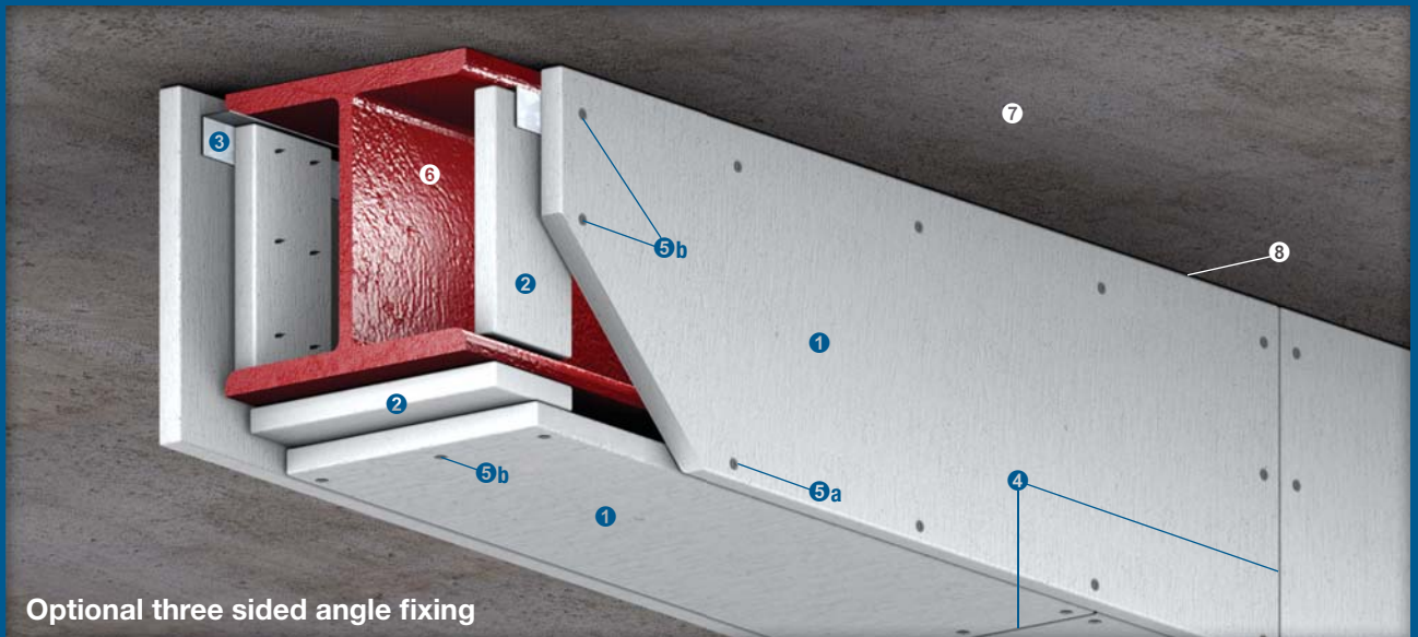
Three sided angle fixing
